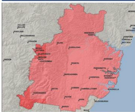
Far future change in maximum temperature
